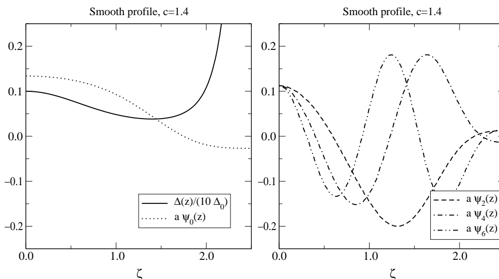
Figure 5: Left: The fundamental mode \psi_0(z) and the profile \Delta(z) for the smooth wave function, eq. (5.10), at c = M/m = 1.4, R = 2.5/m , and a specific a (see table 2). The horizontal axis is for \zeta = zm . Right: the first excited even modes.
