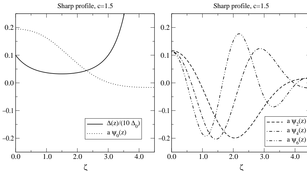
Figure 4: Left: The fundamental mode \psi_0(z) and the profile \Delta(z) for the sharp wave function, eq. (5.4), at c = M/m = 1.5 , R = 4.5/m , and a specific a (see table 1). The horizontal axis is for \zeta = zm . Right: the first excited even modes.
