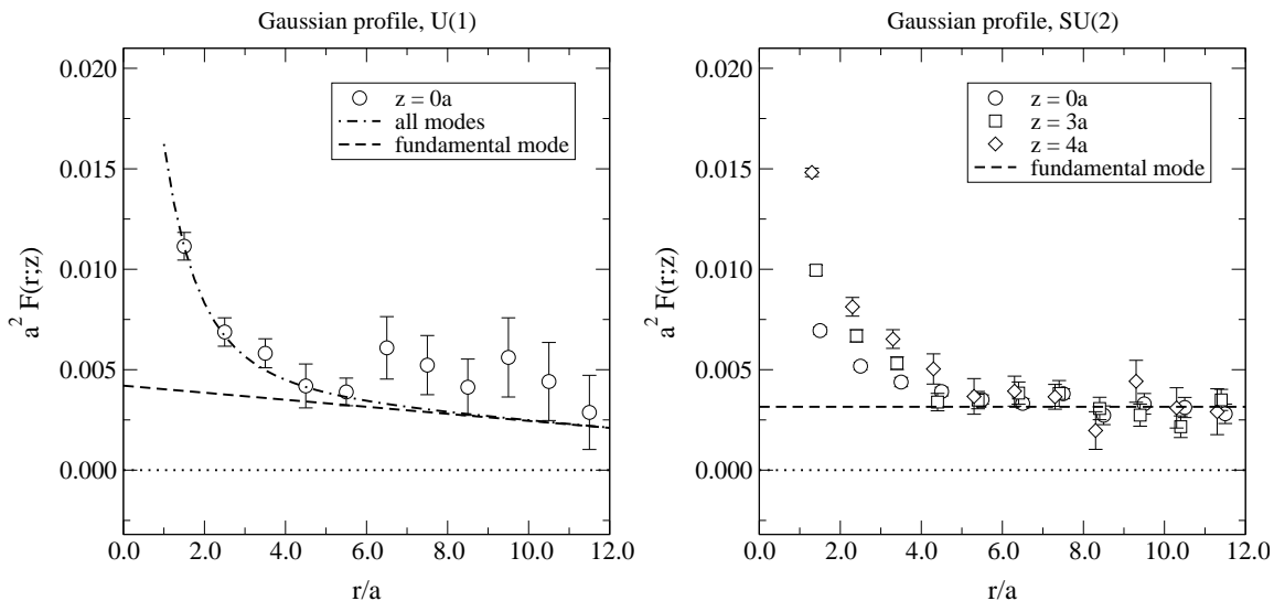
Figure 1: The force F(r; z) for the gaussian weight function, eq. (5.1), at different fixed values of z , in the abelian (left; volume = 48^2 \times 14 ) and non-abelian cases (right; volume = 24^2 \times 14 ). The perturbative values are also shown. The abelian case has a finite slope because of the periodicity discussed around eq. (4.10).
