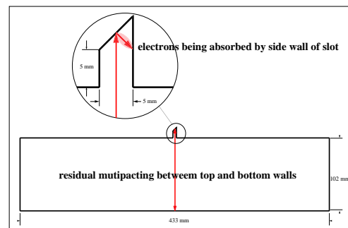
Figure 5: Suppressing multipacting by opening a slot on the top wall along the center plane. Tiltting the ceiling of the slot by 45° provides further suppression by deviating the residual secondary electrons to the side wall of the slot.
