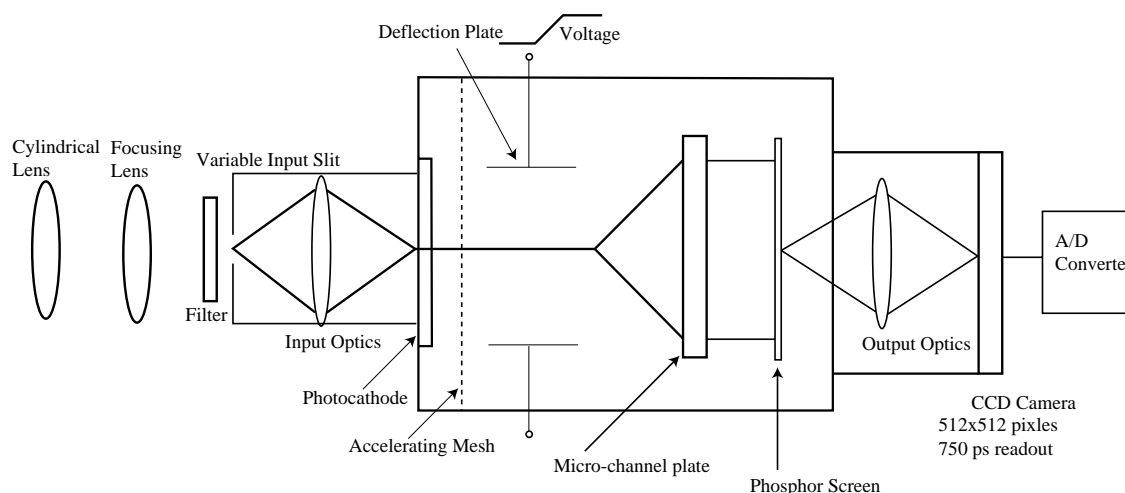
Figure 1. The layout of the various components of the Hamamatsu streak camera.
