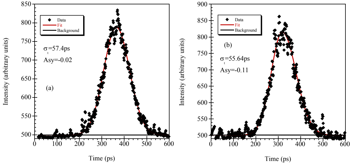
FIG. 2 (color). Two sample longitudinal profiles of the trailing bunch distribution measured by the streak camera. The current of the main bunch for both profile is 20mA and the time spacing between the main and trailing bunch is (a) 56ns (28 RF buckets) and (b) 2ns (one RF bucket).
