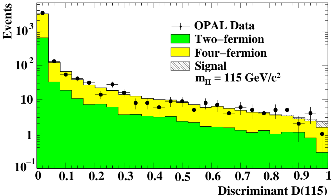
Figure 6: Four-Jet Channel: Distribution of the final discriminating function for a hypothetical m_H=115 GeV/c 2 signal added to the expectations from SM backgrounds.
