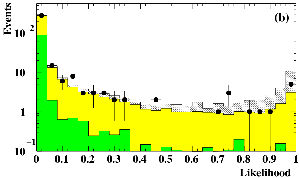
Figure 11: Tau channels: Distributions of the two likelihood output variables (a) \mathcal{L}(\tau\tau q\bar{q}) and (b) \mathcal{L}(b\bar{b}\tau\tau) .
