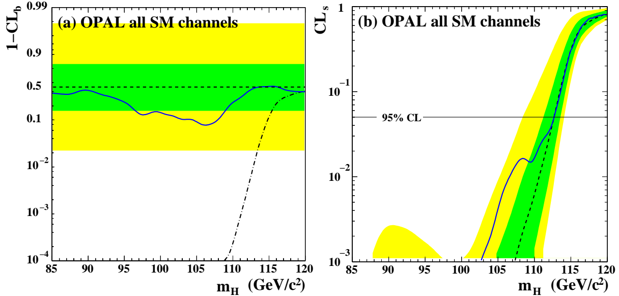
Figure 19: For all search channels combined: (a) The confidence level 1-CL_b , as a function of the Higgs boson test mass. The median expectation in the presence of a signal is presented with the dash-dotted line. (b) The confidence level ratio CL_s=CL_{s+b}/CL_b versus the Higgs boson test-mass. The observations for the data are shown with solid lines. The shaded bands indicate the 68% and 95% probability intervals, with respect to the median expectation in the absence of a signal (dashed line).
