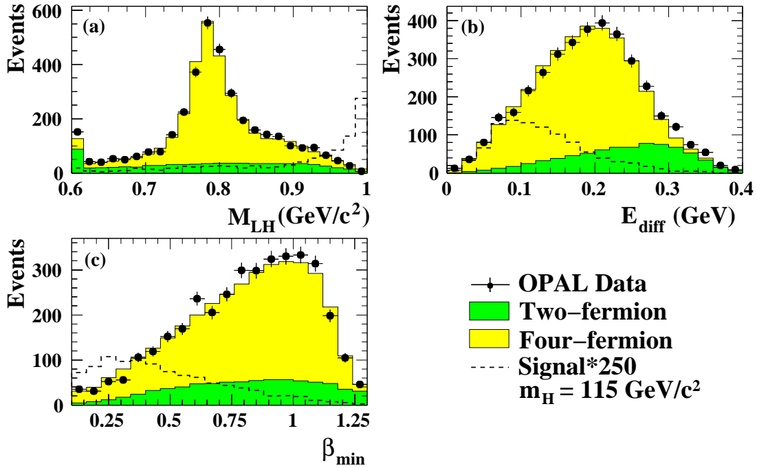
Figure 5: Four-Jet Channel: Distributions of the variables used as input to the likelihood function \mathcal{L}_2 ; (a) M_{LH} , (b) E_{diff} , and (c) \beta_{min} .
