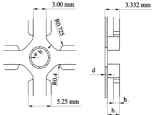
Figure 2: Geometry of the XDSs cell and damping waveguides.
