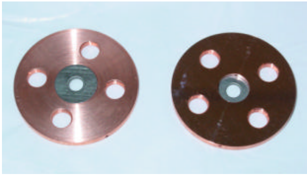
Figure 4: Tungsten irises in copper cells of tungsten-iris structure.
