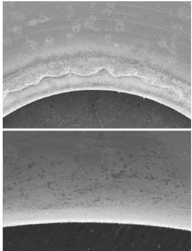
Figure 3: SEM images of the copper (upper) and tungsten (lower) irises. The tungsten image was taken at a higher magnification – the radii are the same.
