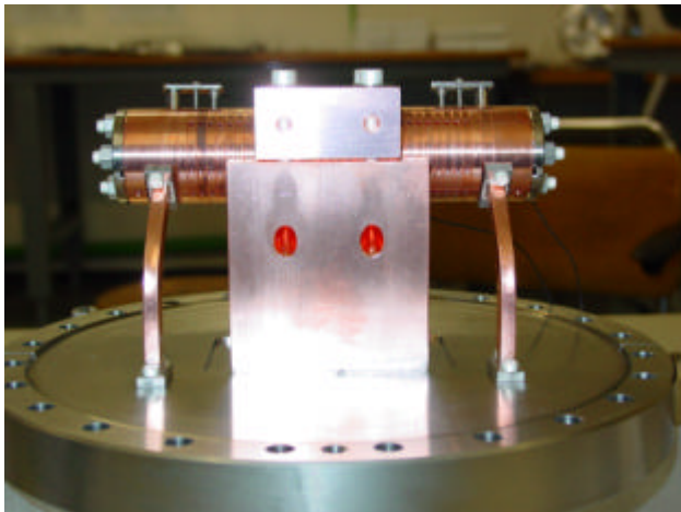
Figure 5: Tungsten iris structure mounted on the vacuum tank cover-plate. The structure is held and cooled by the copper block in the middle of the structure.
