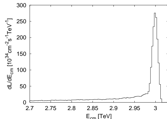
Figure 1: The luminosity spectrum for the perfect machine.
