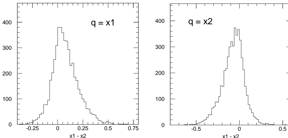
Figure 3: Difference x_1 - x_2 when the quark is picked up from the proton labelled “1” (left plot) and “2” (right plot).
