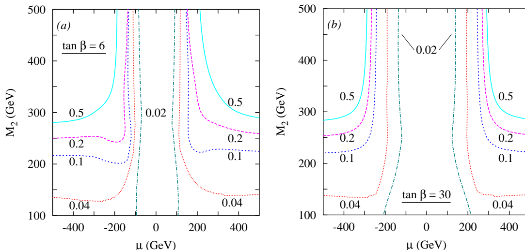
Figure 14: Contours for the branching fraction of a 300 GeV stop ( \tilde{t}_L ) into the R -parity-violating channel. The unification relation between the gaugino masses has been assumed. The value of the R -violating coupling ( \lambda'_{231} = 0.16 ) is the minimum necessary for a determination \lambda' to an accuracy of 5% (see figure 6). The left and right panels correspond to two different values of \tan \beta .
