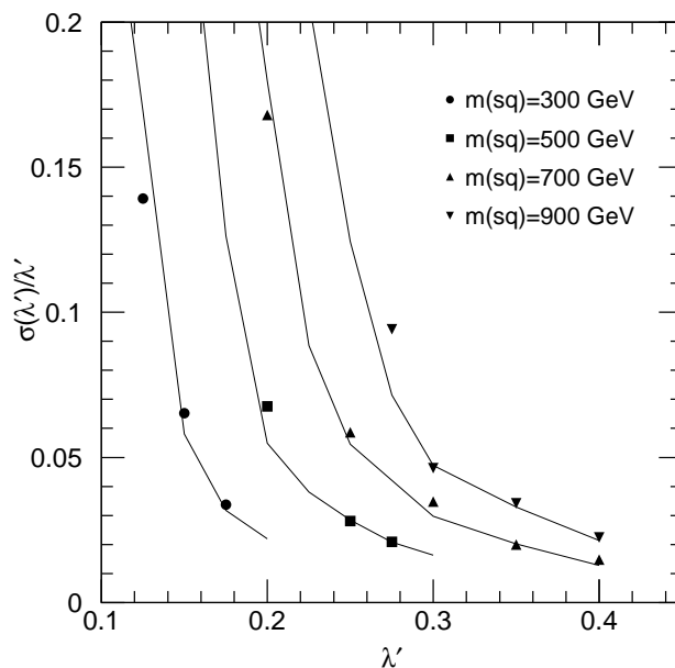
Figure 12: Curves of \sigma(\lambda')/\lambda' as a function of \lambda' for an integrated luminosity of 100\text{ fb}^{-1} and for four different squark masses. The full lines give the resolution obtained at parton level, and the points are the results of the full event simulation.
