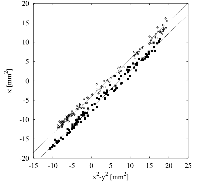
FIG. 3: Quadrupole moment (uncorrected) versus expected beam position contribution. The squares and circles represent measurements made with the same pick-up on two different beams. The slope of the line is the same in both cases, and is very close to one (0.983).
