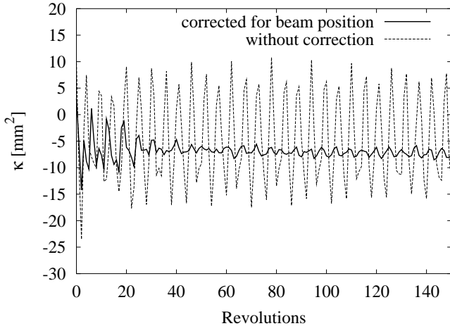
FIG. 2: Quadrupole moment \kappa measured with a PS pick-up immediately after injection, with and without correction for beam position. The initial beam-size oscillation is clearly visible in the corrected signal. Note the fast decoherence of beam size oscillations, due to direct space charge.
