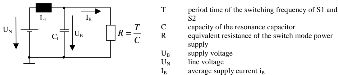
Figure 2: Equivalent circuit of the power supply
