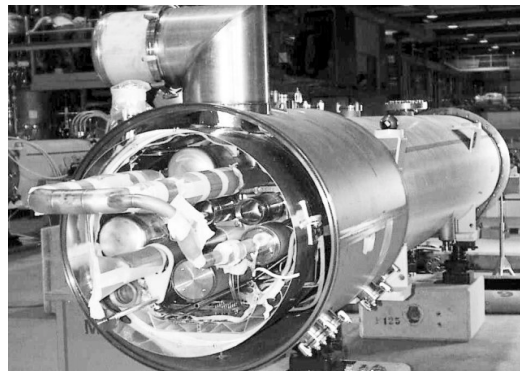
Figure 1: LHC Arc Short Straight Section Prototype.
