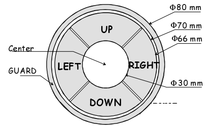
Figure 1: Layout of the ‘Centroid’ detector.
