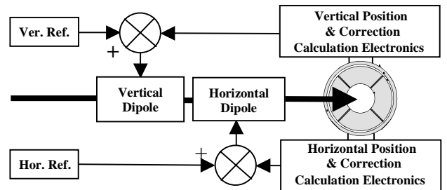
Figure 2: Block schematic of the feedback system.
