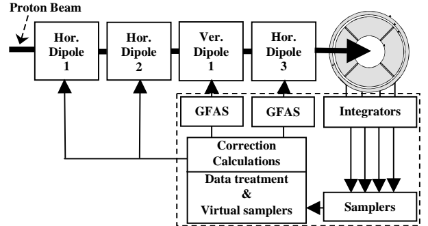
Figure 4: Block schematic of the feed forward system.
