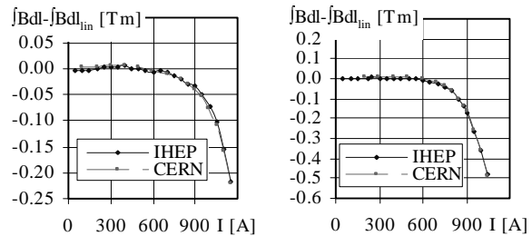
Figure 3: Nonlinearity of magnetisation curves, left: MSIB01, right: MSDC01
