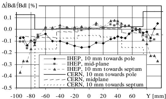
Figure 5: Transverse field homogeneity of MSDC01
