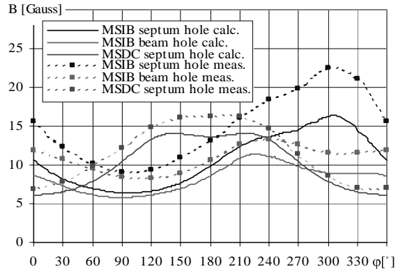
Figure 6: Field in beam and septum holes
