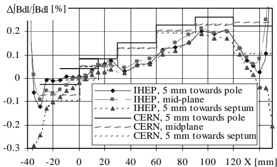
Figure 4: Transverse field homogeneity of MSIB01
