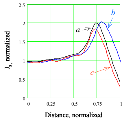
Figure 2. Surface magnetic field profiles for three DFC versions.
