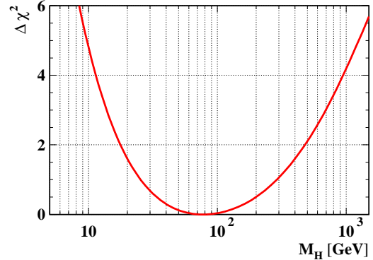
Figure 2. First \Delta\chi^2 = \chi^2 - \chi_{\text{min}}^2 vs m_H fit results plot including the CDF value of m_t .
