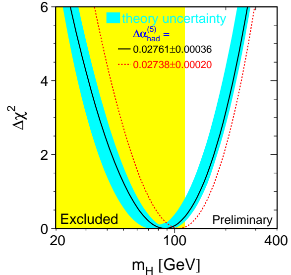
Figure 8. \Delta\chi^2 = \chi^2 - \chi_{\min}^2 vs. m_H curve. The line is the result of the fit using all data; the band represents an estimate of the theoretical error due to missing higher order corrections. The vertical band shows the 95% CL exclusion limit on m_H from the direct search.
