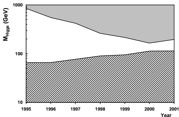
Figure 11. Variation over seven years of the lower limit on the Higgs boson mass from direct searches (dashed area) compared to the upper limit derived from electroweak fits (shaded area).
