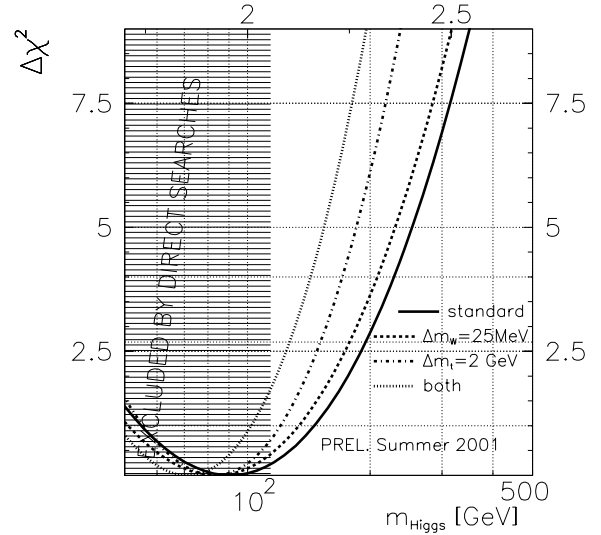
Figure 10. \Delta\chi^2 curves for a precision of 25 MeV on m_W and 2 GeV on m_t . Central values of m_W and m_t are kept unchanged.
