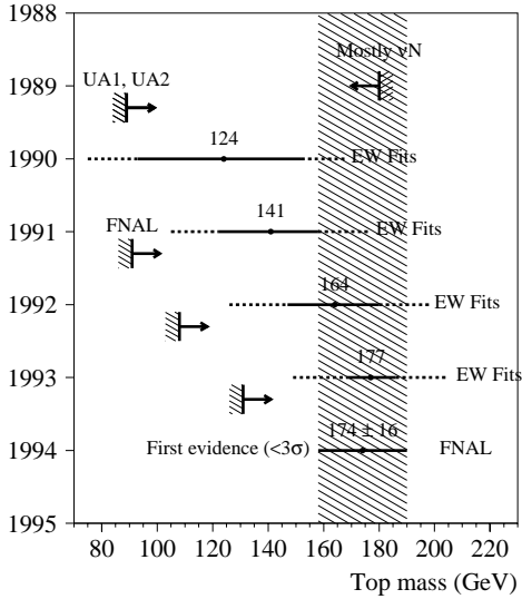
Figure 1. Time evolution of the top quark mass derived from electroweak fits, compared to direct searches results.
