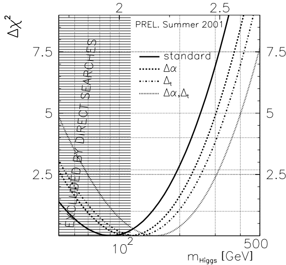
Figure 9. \Delta\chi^2 for one sigma change of \Delta\alpha_{\text{had}}^{(5)}(m_Z^2) or m_t and both.
