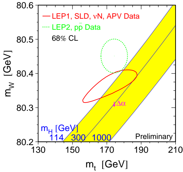
Figure 7. The comparison of the indirect measurements of m_W and m_t (solid contour) and the direct measurements (dashed contour). In both cases the 68% CL contours are plotted. Also shown is the Standard Model relationship for the masses as a function of the Higgs mass.
