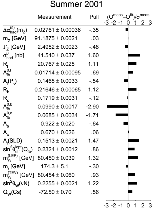
Figure 5. Summary of measurements that enter the electroweak fits together with their pull.
