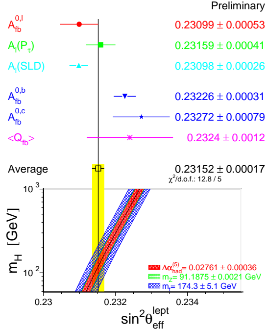
Figure 3. Comparison of several determinations of \sin^2 \theta_{\text{eff}}^{\text{lept}} from asymmetries. Also shown is the prediction of the Standard Model as a function of m_H . The width of the Standard Model band is due to the uncertainties in \Delta\alpha_{\text{had}}^{(5)} , m_Z and m_t . The total width of the band is the linear sum of these effects.
