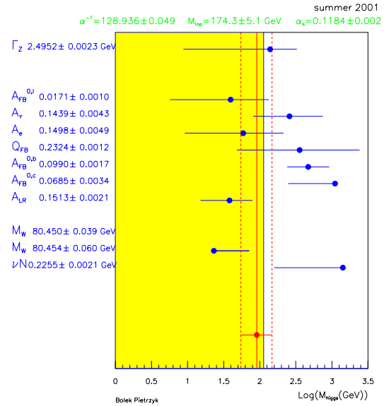
Figure 6. Constraints on \log m_H from various observables.
