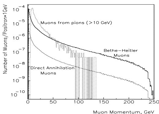
Figure 5: Cross-sections for muon production
