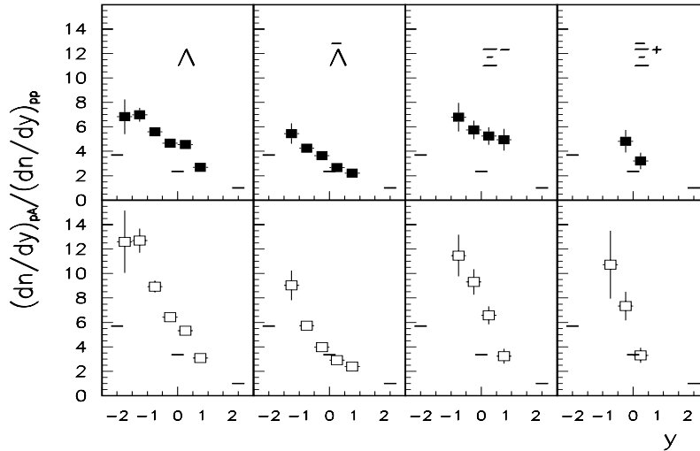
Figure 5. Ratios of hyperon multiplicities in centrality selected p+Pb and minimum bias p+p collisions versus rapidity [2]. The experimental results for the first ( \langle \nu \rangle = 3.7 ) and the second ( \langle \nu \rangle = 5.7 ) centrality bin, are shown by full and open squares, respectively. The predictions of the WNM at backward, central and forward rapidities are indicated by the solid lines.
