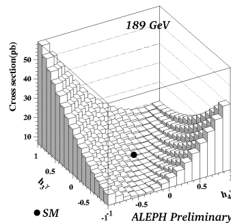
Figure 5: Variation of the Z\gamma cross-section with respect to (h_3^V, h_4^V) .
