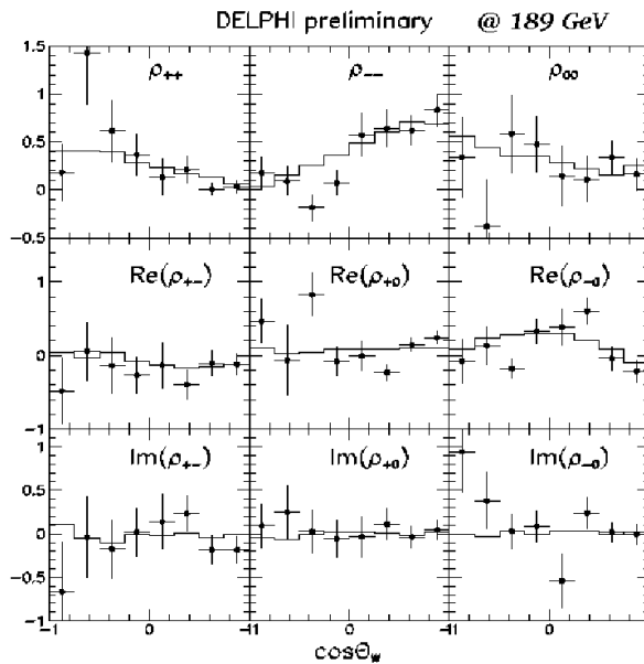
Figure 1: The SDM elements for the W^+W^- production.
