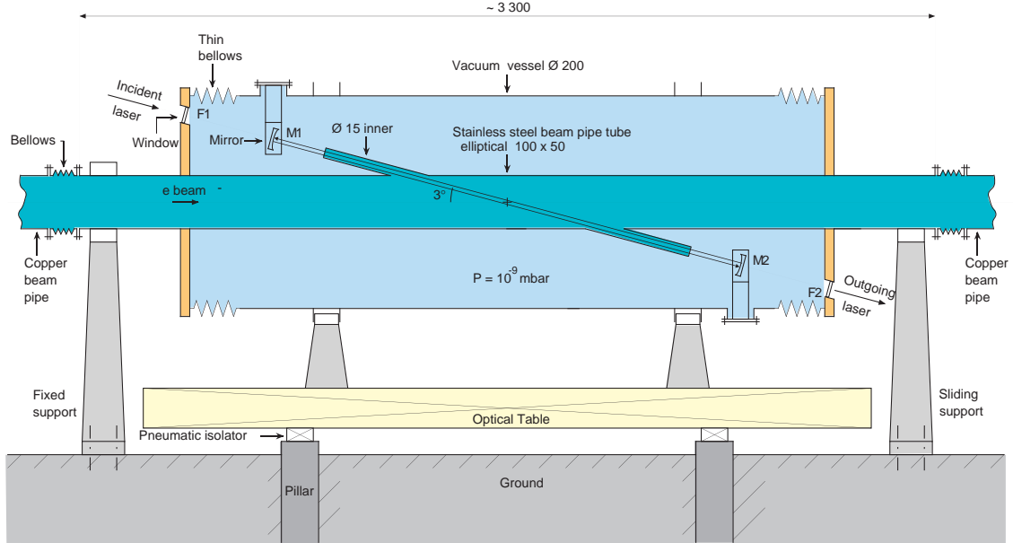
Figure 2: Schematic layout of the new longitudinal polarimeter.
