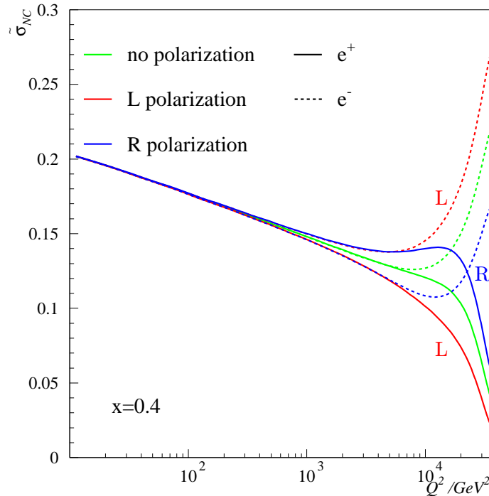
Figure 1: The reduced e^\pm p neutral current (NC) cross-section as a function of Q^2 for different electron polarizations. The cross-section is largest (smallest) for left(L) polarization in the e^-p ( e^+p ) collisions.
