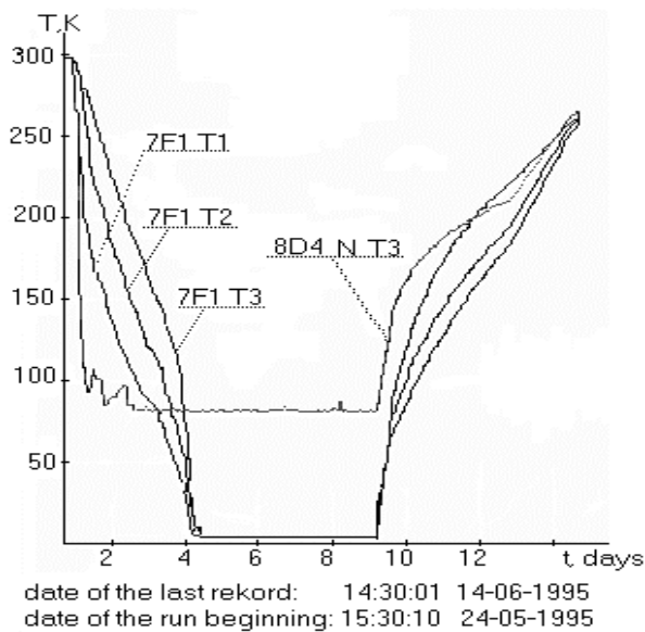
Fig.3: Temperature change for 4 sensors during the Nuclotron run.
