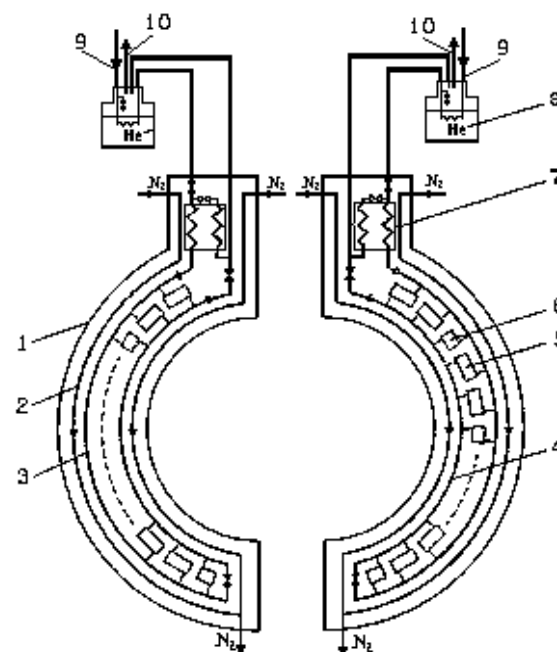
Figure 1: General scheme of the Nuclotron cryogenics: 1 - vacuum shell; 2 - heat shield; 3 - supply header; 4 - return header; 5 - dipole magnet; 6 - quadrupole magnet; 7 - subcooler; 8 - separator; 9 - helium flow from the refrigerator; 10 - return helium flow to the refrigerator;
