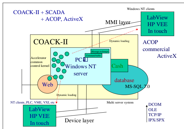
Fig.1 COACK-II system
