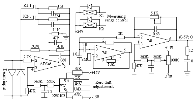
Figure 1: Basic circuit of IVC with 50Hz filter
