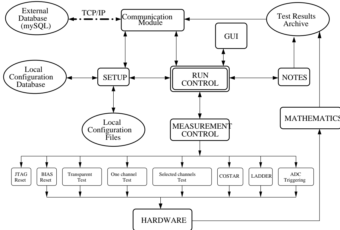
Figure 2. Measurement program architecture
