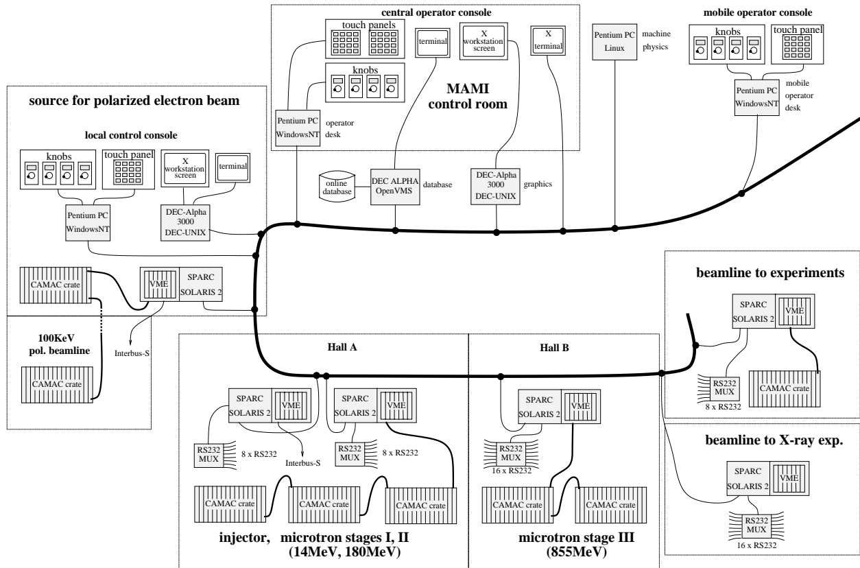
Figure 1: Topology of the MAMI Control System
