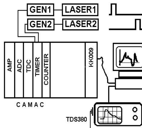
Figure 2: The electronics scheme.
