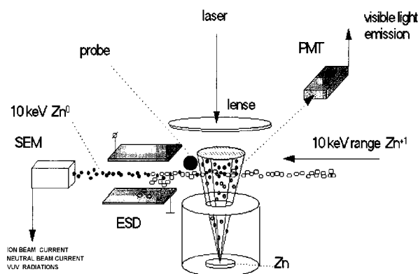
Figure 1: The experimental setup scheme.
