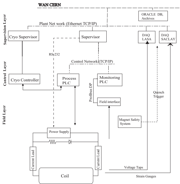
Figure 1: Proposed architecture.
