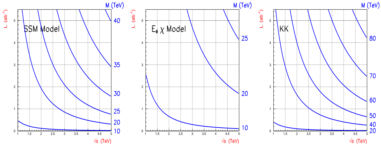
FIG. 1: The 95% C.L. sensitivity contours in the L vs. \sqrt{s} plane for different values of M_{Z'} in the SSM model (left) and in the E_6 \chi model (center) and for different values of the compactification scale M in a five dimensional extension of the SM with fermions on the boundary (right).
