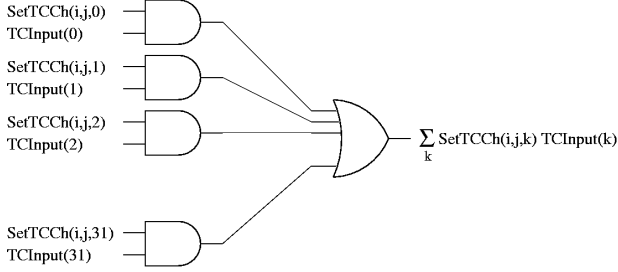
Figure 4: Tile Calorimeter coincidence implementation. For a given Pad and a given threshold a muon candidate is accepted if one hit is found in one of the corresponding Tile Calorimeter trigger towers.
