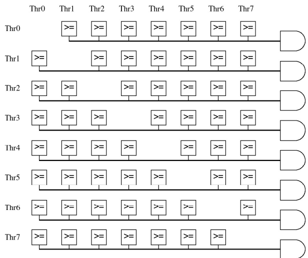
Figure 6: 1 st highest threshold search implementation. For each Pad the muon candidate threshold is compared with the thresholds of all the other Pads and the comparison output are ANDed for each Pad.
