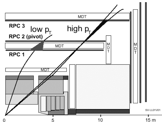
Figure 1: Trigger principle for the ATLAS first level muon trigger in the barrel. The selection is performed using three dedicated trigger chambers. For the low- p_T trigger if an hit is found in RPC2, an hit is searched for in the RPC1 trigger station inside a road defined by the p_T cut. The same algorithm is applied for the high p_T threshold using the low- p_T trigger output and the RPC3 trigger station.
