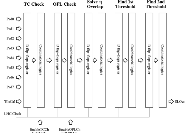
Figure 3: Block diagram of the architecture of the Sector Logic chip. The Sector Logic algorithm is implemented with a five steps pipeline, each step of the pipeline implementing one task of the algorithm.
