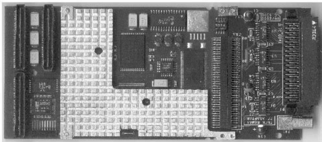
Figure 8: Layout of the MFCC with the FE adaptor card translating the MFCC Sector Logic output to LVDS logic levels used to interface the Sector Logic demonstrator with the MUCTPI prototype.
