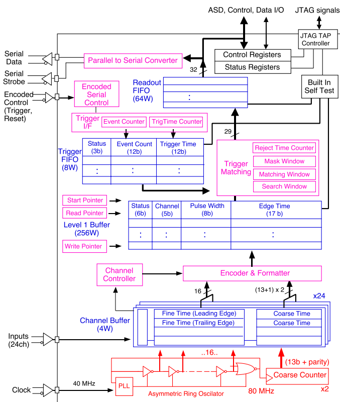
Fig. 1 Block diagram of the AMT-2 chip.
