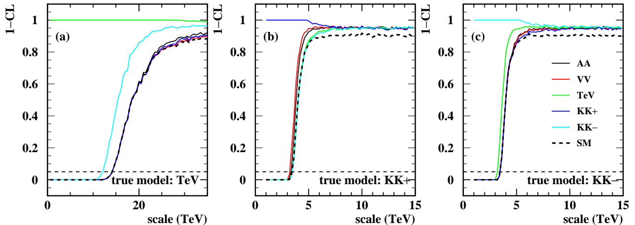
FIG. 6: Expected 1-\text{CL} at a 500 GeV linear collider with 100 \text{ fb}^{-1} luminosity after combining the three lepton pair final states, as a function of the scale parameter of the true model, assumed to be (a) TeV-scale extra dimensions, large extra dimension with dominant contribution from KK excitations of the graviton with (b) \lambda=+1 and (c) \lambda=-1 using the notation of Hewett, for various tested models. AA and VV stands for composite lepton models with axial-axial and vector-vector couplings. The large extra dimension scenario with dominant contribution from string Regge states is omitted from this combined plot due to the lack of calculations for the muon and tau pair final states.
