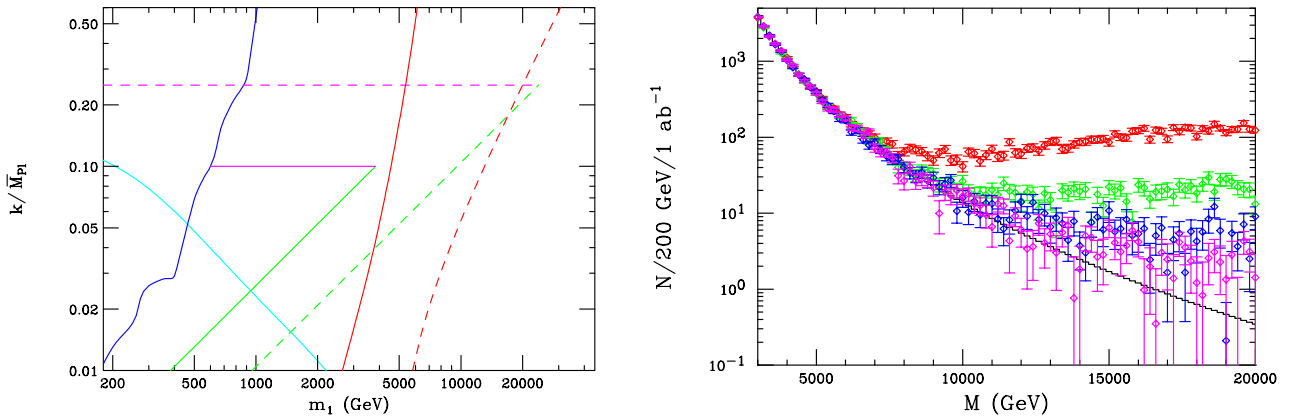
FIG. 3: (Left) Allowed regions of the RS model parameter space; m_1 is the lightest KK graviton mass. Current Tevatron (blue) and precision measurements (cyan) forbid regions to the left of their specific curves. The horizontal magenta solid (dashed) lines form the upper bound of the region when c = k/\overline{M}_* = 0.10 (0.25) while the solid (dashed) green curve is the corresponding lower bound when \Lambda_\pi = 10 (25) TeV. The solid (dashed) red curve is the reach of the LHC (CLIC) with 100 fb^{-1} ( \sqrt{s} = 5 TeV with 1 ab^{-1} ). (Right) Event rate per 200 GeV mass bin for the Drell-Yan process as a function of the lepton pair invariant mass at a \sqrt{s} = 200 TeV stage II VLHC. A rapidity cut \eta < 2.5 on both leptons has been applied. The solid histogram is the SM background in both cases whereas the ‘data’ points are the predictions of the ADD model. The red, green, blue and magenta points correspond to a Hewett cutoff scale of M_s = 20, 25, 30 or 35 TeV, respectively.
