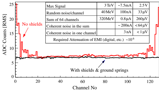
Figure 14. Coherent noise measured for the 128-channel LAr FEB (front-end readout board). Critical role of shielding and ground springs at the input connectors is illustrated, resulting in a coherent noise of only \sim 1 microvolt/channel.
