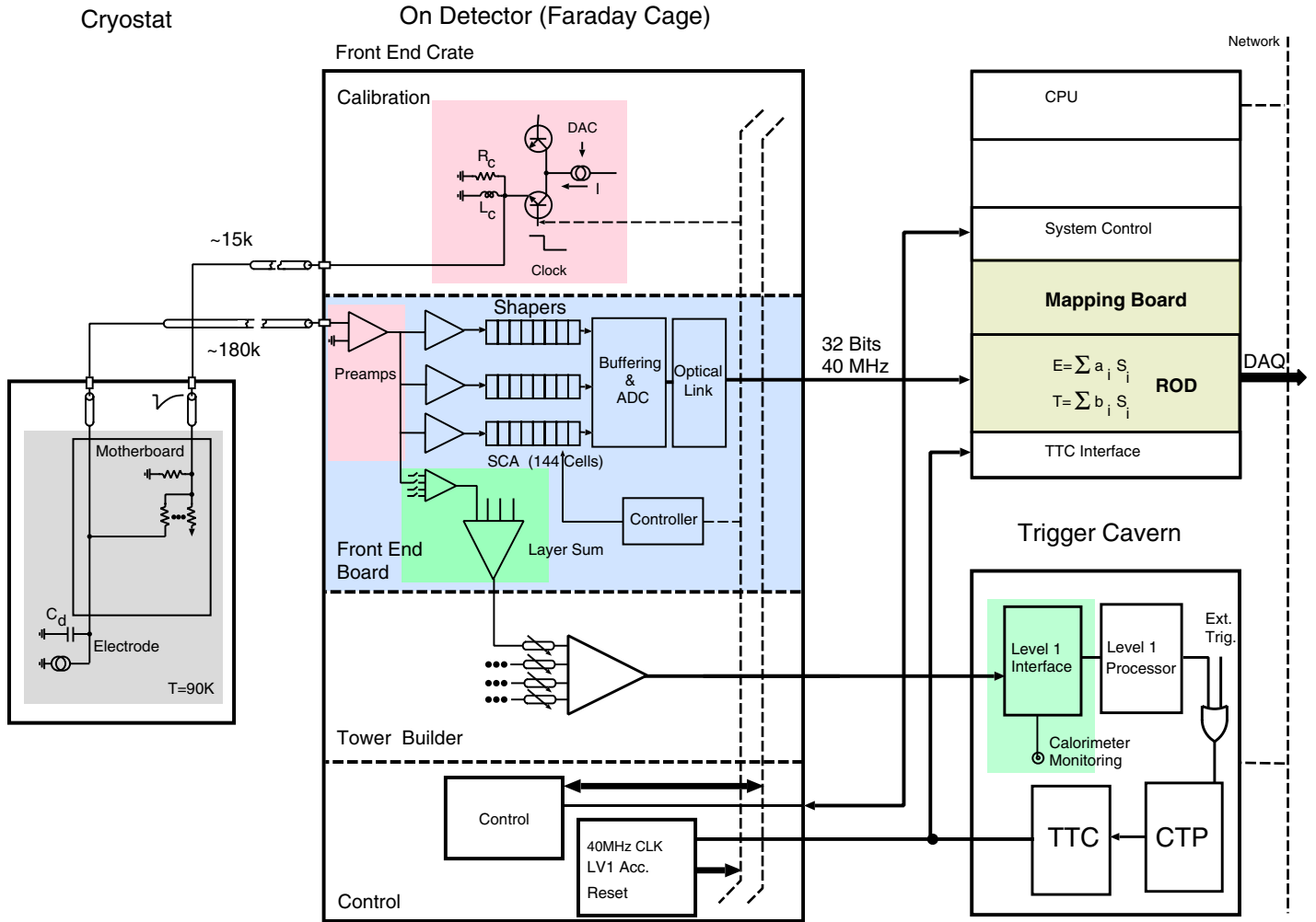
Figure 11. Readout chain of the ATLAS liquid argon calorimeter. After the preamplifiers, the readout chain is identical for all the liquid argon calorimeters. The end-cap hadron calorimeter has preamplifiers based on GaAs technology at the electrodes inside the cryostat. Each preamplifier output is split into three shaping amplifiers with different gains and analog (switched capacitor) memories, and then digitized with 12 bit resolution. Data are transferred from the detector via one optical link for every 128 signal channels.
