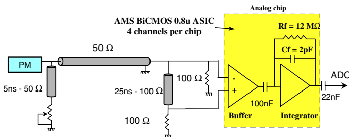
Figure 2. Principle of the Integrator Filter for the LHCb ECAL and HCAL. The exponentially decaying signal is first clipped at the photomultiplier output to 5 ns. The integrator receives the clipped signal, and then after 25 ns the same but with opposite polarity, to provide an output with a flat top, which returns to zero, as shown in Fig. 3.
