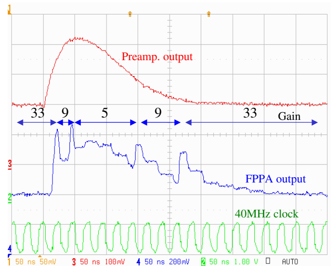
Figure 7. Waveform at the output of the analog multiplexer of CMS ECAL floating point preamplifier (FPPA). It consists of consecutive samples every 25 ns, each sample taken from one of the four amplifiers which provides the best precision for a given signal amplitude (a short transient is superposed as boundaries between different gains are crossed; sample magnitudes are measured at points in between the transients).
