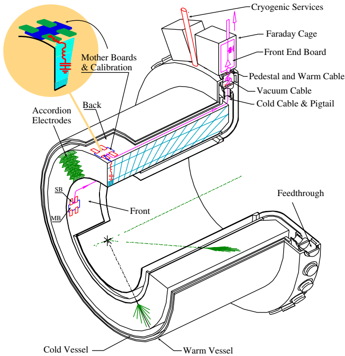
Figure 10. An illustration of the readout of the ATLAS liquid argon (barrel) EM calorimeter. The crates (“Faraday Cage”) containing all the functions outlined in the lower half of Fig. 11 are mounted directly on signal feedthroughs.
