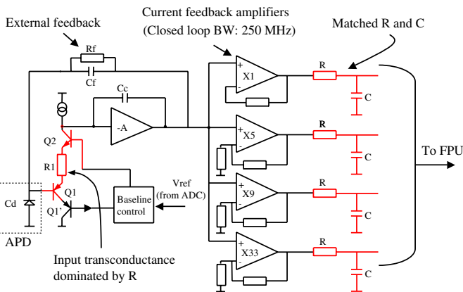
Figure 6. Circuit topology of the CMS ECAL floating point preamplifier. Four samples at different gains are stored every 25 ns. The sample with the highest gain below saturation is selected and fed to the ADC via a multiplexer, resulting in a waveform as in Fig. 7.
