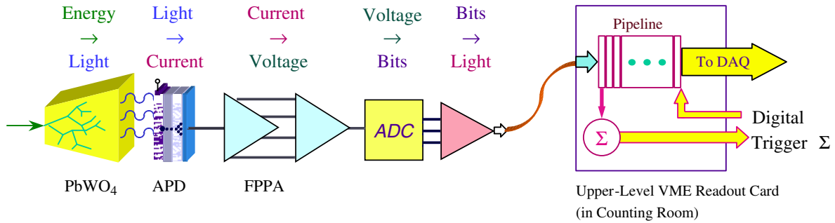
Figure 4. Readout chain for the CMS electromagnetic calorimeter. Preamplifier with range selection (Floating Point Preamplifier – FPPA) and analog-to-digital converter are located at the detector ( \text{PbWO}_4 crystals with avalanche photodiode readout). There is 1 fiber per crystal for data transmission from the detector. Digital pipelines are in the counting room.
