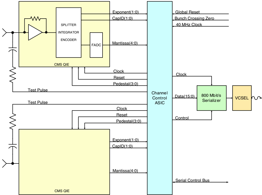
Figure 8. Block diagram of the CMS hadron tile calorimeter readout. The front end, including analog-to-digital conversion, is based on the pipelined multi-ranging integrator and encoder (ref. ), known as “QIE”. The encoder is based on a multi-ranging current splitter and a nonlinear flash ADC. Encoded samples are serialized and transferred from the detector by (one) optical link for every two channels.
