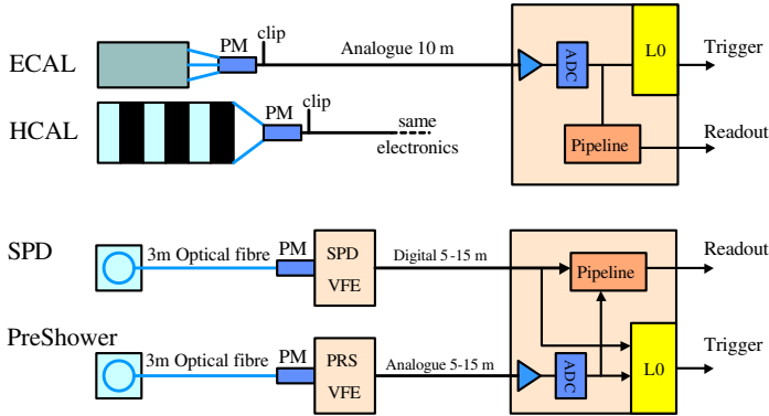
Figure 1. Front-End Electronics for LHC calorimeters. (Design of the Integrator Filter for ECAL and HCAL is by LAL Orsay, and VFE for the Scintillator Pad Detector and for the Preshower is by LPC Clermont-Ferrand.)
