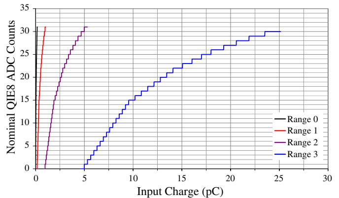
Figure 9. Response of the CMS charge integrator encoder (QIE) over the four gain ranges.
