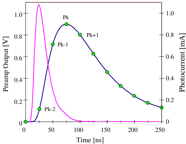
Figure 5. \text{PbWO}_4 /APD signal before and after shaping. Sampling points every 25 ns are indicated.
