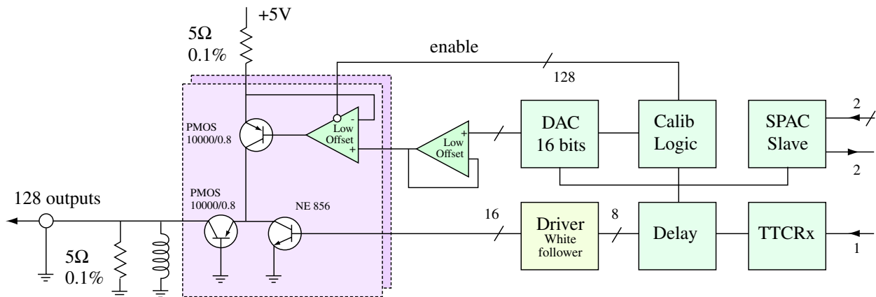
Figure 12. Calibration signal generator. A dc current controlled to 0.1% is switched off to generate on an LR network an exponentially decaying current pulse which approximates closely (within the shaping time) the calorimeter signal.
