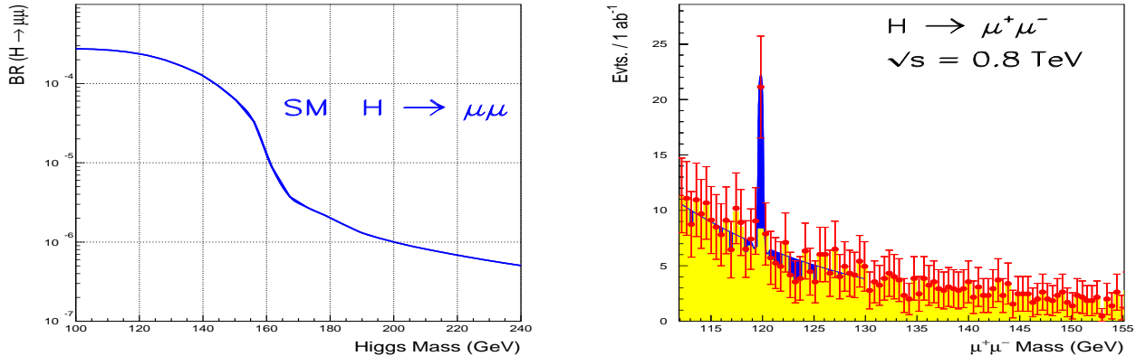
FIG. 1: Left: SM prediction for \text{BR}(H \rightarrow \mu^+\mu^-) as a function of the Higgs boson mass. Right: distribution of the di-muon invariant mass M_{\mu\mu} for M_H=120 GeV. The points with error bars represent 1 \text{ ab}^{-1} of data at \sqrt{s}=0.8 TeV and the continuous line the result of the fit used to extract the number of signal events.
