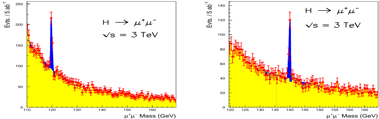
FIG. 2: Distribution of the di-muon invariant mass M_{\mu\mu} for two data sets with M_H=120 GeV (left) and M_H=140 GeV (right). The points with error bars represent 5 \text{ ab}^{-1} of data at \sqrt{s}=3 TeV and the continuous lines the results of the fits used to extract the numbers of signal events.
