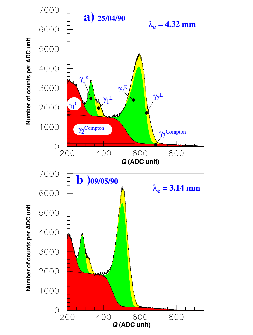
Figure 5: Comparison of the analytical function S_{Bi}(Q) with spectra of a ^{207}\text{Bi} probe with 6 mm gap. a) data of 25/04/90, b) data of 09/05/90. Areas corresponding to the three electron conversion mechanisms (K, L, Compton) are filled with different shades.
