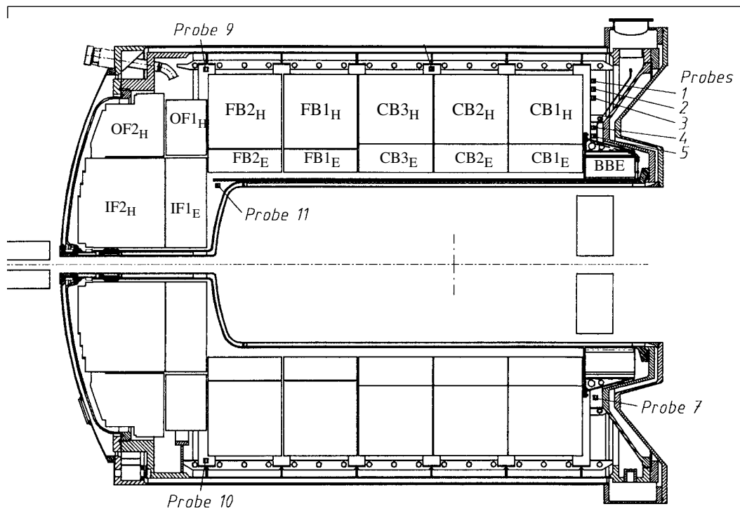
Figure 2: Location of purity probes inside the H1 LAr cryostat.
