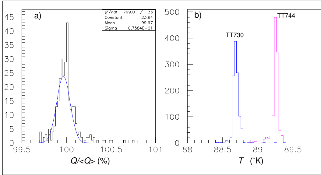
Figure 7: October 99: a) thermal fluctuation of purity ( Q/\langle Q \rangle 6mm probe; 1 MeV estimator); b) temperature distributions measured in 2 points of the cryostat (probes are not calibrated absolutely).
