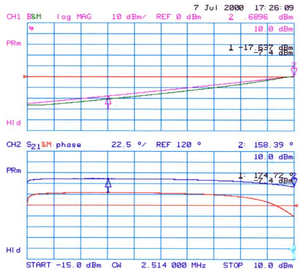
Figure 5: Coalescing Cavity Power Sweep with (magenta) and without (green) feedback.
