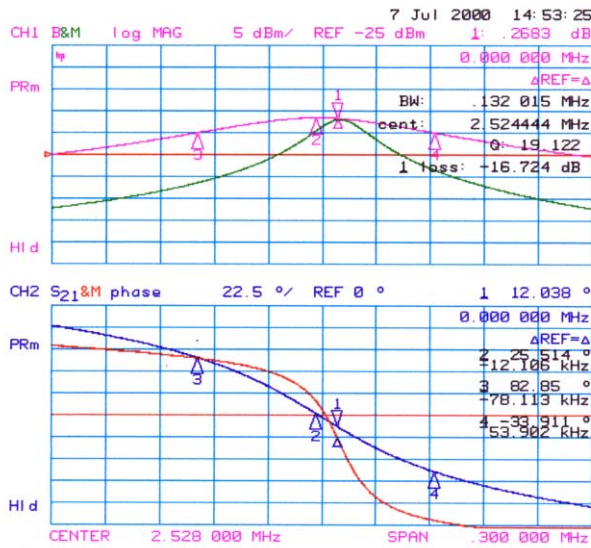
Figure 4: Coalescing Cavity Response with (magenta) and without (green) Feedback.
