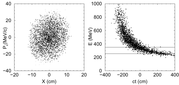
Figure 6: Transverse and longitudinal phase space of muons at the end of the decay channel.
