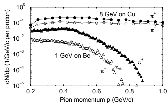
Figure 2: MARS calculated pion spectra (per interacting proton) at the downstream end of a Li-lens for 8-GeV protons on a 15-cm copper target, and 1-GeV protons on a 15-cm beryllium target.
