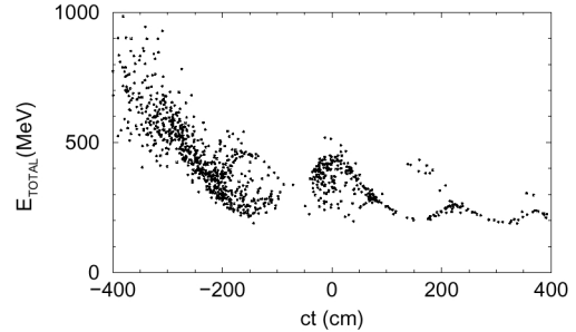
Figure 8: Longitudinal phase space of muons after the bunching.
