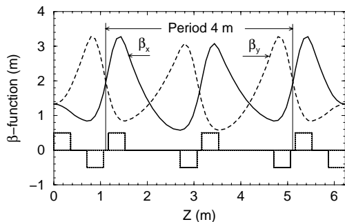
Figure 7: Layout and \beta -functions of the decay channel with bunchers.
