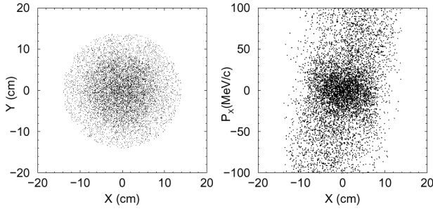
Figure 3: Transverse phase space of pions.
