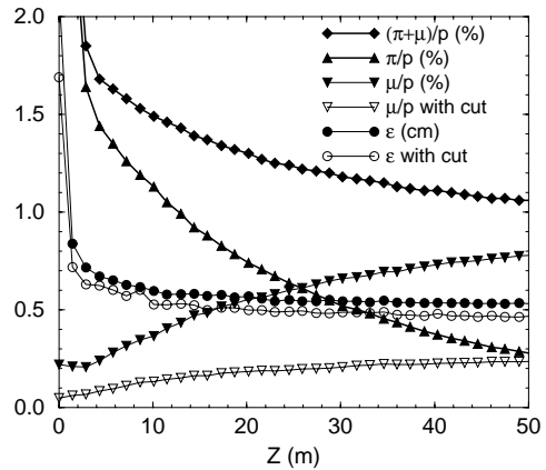
Figure 5: Evolution of the beam parameters in the decay channel.
