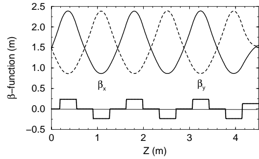
Figure 4: Layout and \beta -functions of the decay channel.
