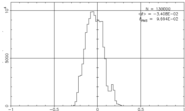
Figure 4: Azimuthal projection of roatated bunch shown in Fig. 3, abscissa in degrees. The rms bunch length in time is 0.64 ns.
