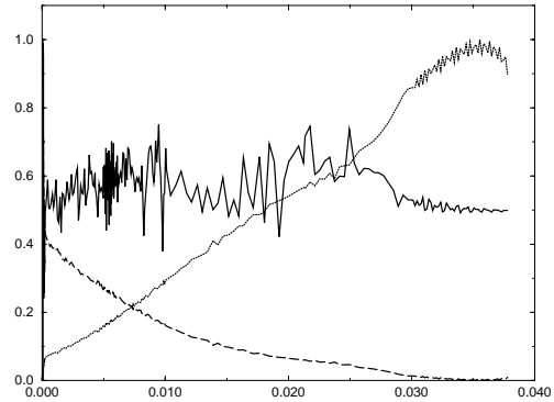
Figure 2: RMS normalized emittance (solid), rms bunch width (dashes), and rms bunch height (fine dots) for the stage one acceleration cycle, all scaled to plot in the range 0 to 1.
