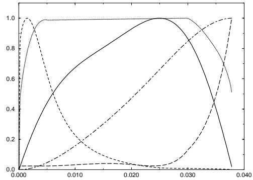
Figure 1: RF parameters during the cycle of the Stage 1 proton driver scaled to the range 0 to 1: V_{rf} (fine dots), p (dash-dot), \dot{p} (solid), \nu_s (short dash), and bucket area (long dash)
