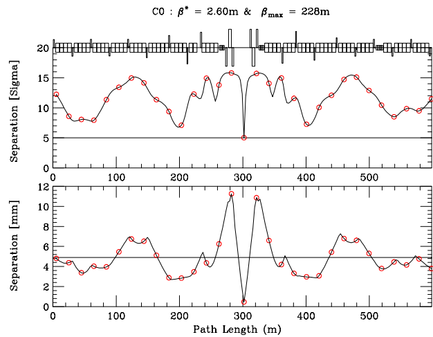
Figure 3: Separation at C0 during B0 & D0 collisions.
