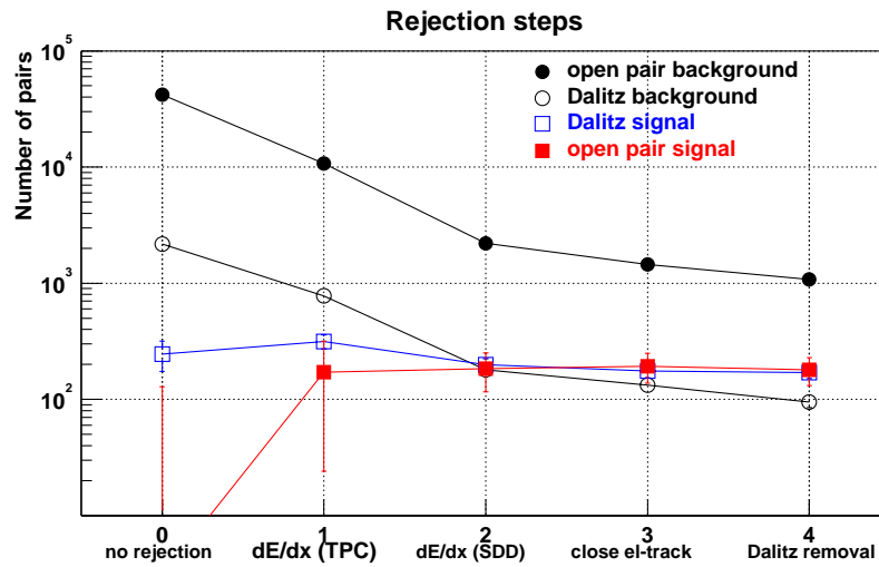
Figure 2: Evolution of the total number of pairs after various rejection steps, shown for the open-pair signal ( m_{ee} > 0.2 \text{ GeV}/c^2 ), open-pair background ( m_{ee} > 0.2 \text{ GeV}/c^2 ), Dalitz signal ( m_{ee} < 0.1 \text{ GeV}/c^2 ) and Dalitz background ( m_{ee} < 0.1 \text{ GeV}/c^2 )
