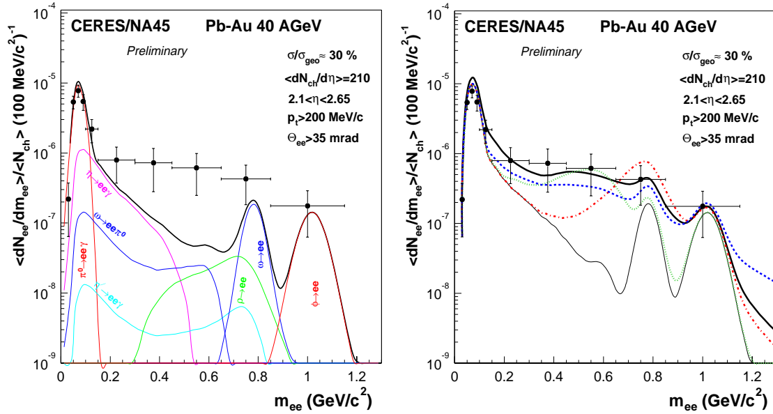
Figure 3: Normalized invariant-mass spectra of e^+e^- pairs at 40 AGeV. Left panel: Comparison of the data to the known hadronic decay sources, showing the individual contributions. Right panel: Comparison of the data to model calculations [10], based either on \pi^+\pi^- annihilation with an unmodified \rho (dashed-dotted), an in-medium dropping \rho mass (dotted) and an in-medium spreaded \rho (thick solid), or on q\bar{q} annihilation in the spirit of hadron-parton duality (dashed); the sum of the hadronic decay sources, but without the \rho , is shown separately (thin solid).
