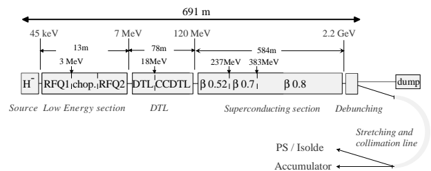
Figure 1: SPL block diagram
