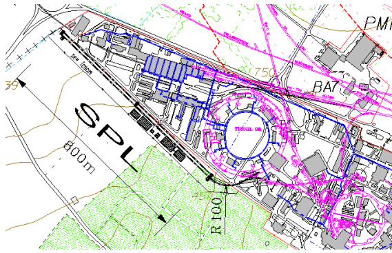
Figure 2: Proton driver complex on the CERN site.
