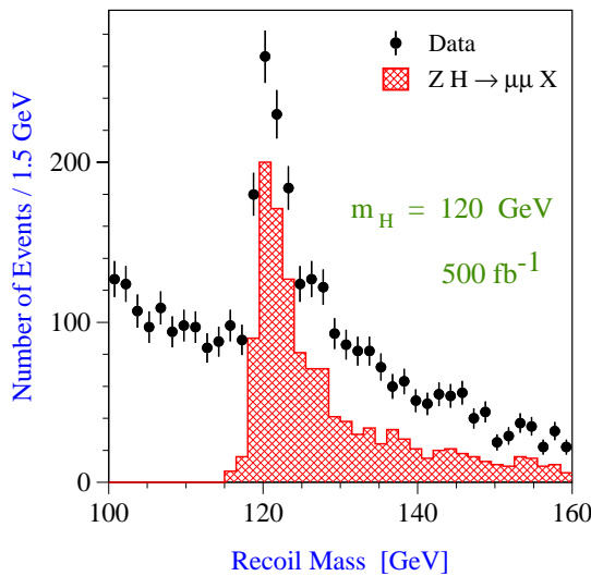
Figure 1: Higgs boson signal in the recoil mass distribution to a muon pair compatible with a Z decay for a simulated Higgs boson mass m_H = 120 GeV and 500 \text{ fb}^{-1} at \sqrt{s} = 350 GeV.
