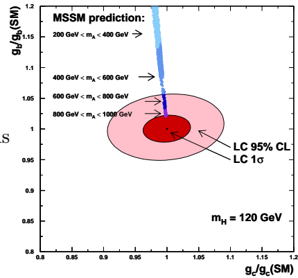
Figure 4: Expected sensitivity of the Higgs couplings g_{Hbb} vs. g_{Hcc} for a Higgs boson mass m_H = 120 \text{ GeV} and 500 \text{ fb}^{-1} .
