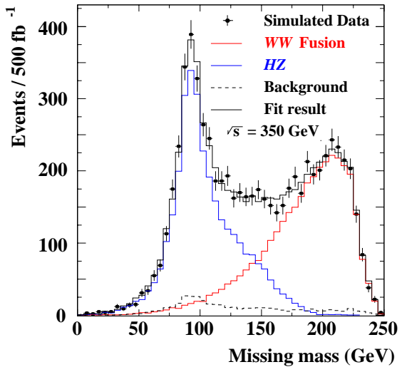
Figure 2: Missing mass distribution in events with two b-jets with an invariant mass compatible with the Higgs boson mass for 500 \text{ fb}^{-1} at \sqrt{s} = 350 GeV.
