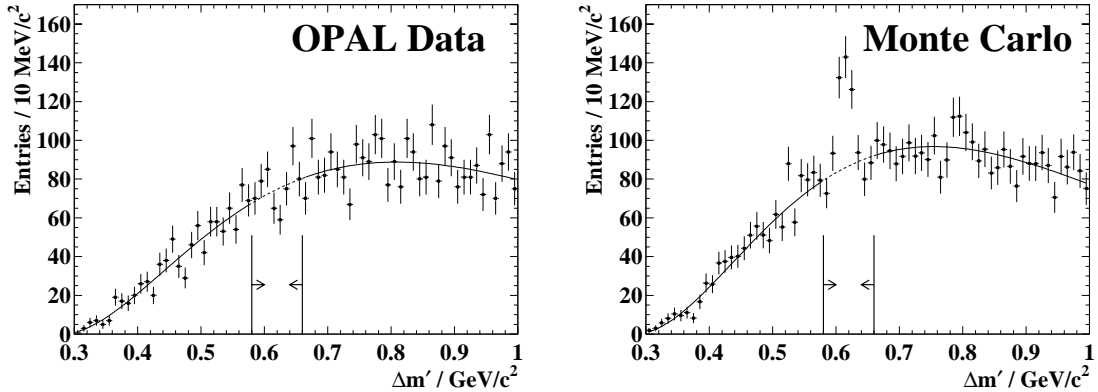
Figure 2: Mass spectrum of D^{*+}\pi^+\pi^- candidates seen by OPAL (left). No narrow resonance is found. An upper limit on the production rate of a possible narrow radial excitation is calculated for a mass inside the mass window represented by the arrows. The right plot shows the corresponding spectrum for a Monte Carlo simulation including a resonance similar to the one reported by DELPHI.
