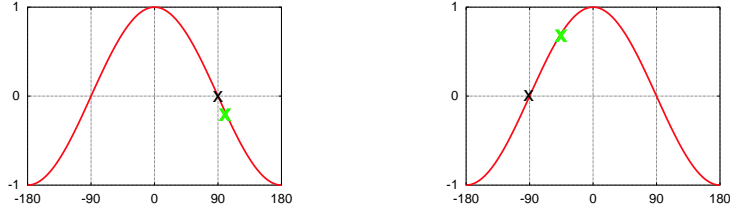
Figure 5: Arrival of bunches with negative phase or energy offset in the debunching (left) and the bunch rotation (right) cavities
