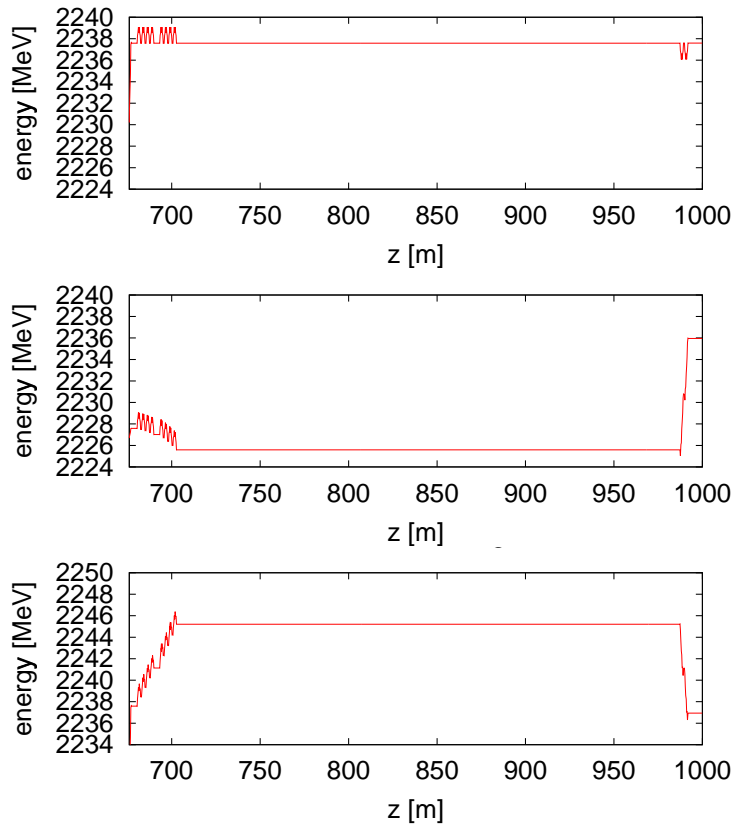
Figure 6: Evolution of average bunch energy in the nominal case (upper), with -10 MeV initial offset (middle), and with +7.5^\circ initial offset (lower).
