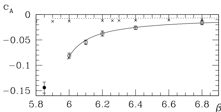
Figure 4: The result for c_A at \beta = 5.85 (filled circle) compared with the results from ref. [37] (open circles). The solid curve is the interpolating formula valid for 6.0 \leq \beta . The dashed curve denotes perturbation theory in the bare coupling, whereas the crosses represent the estimates in mean-field improved perturbation theory.
