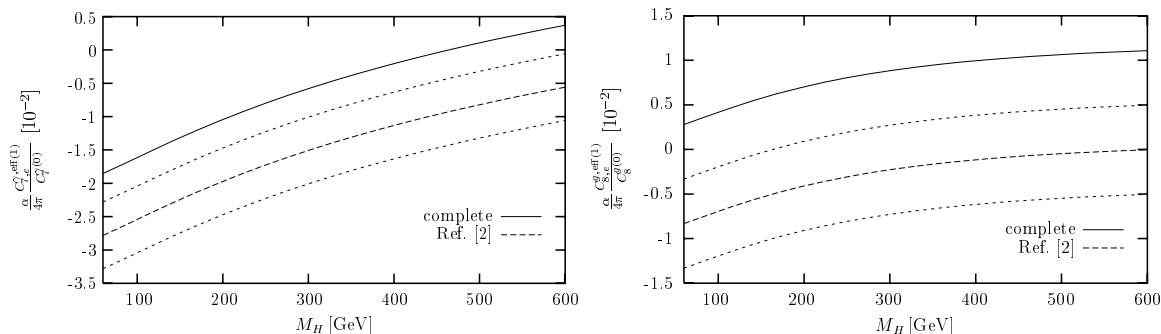
Figure 2: Electroweak corrections to the Wilson coefficients C_7^\gamma(M_W) and C_8^g(M_W) . The dashed lines represent the results of [2] with their error estimates, the solid lines the complete corrections to the Wilson coefficients at M_W .
