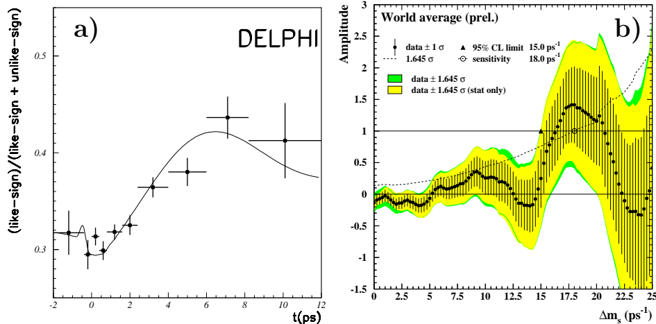
Figure 5: a) Fraction of events in which the oscillation B_d^0 - \bar{B}_d^0 took place as a function of the reconstructed proper time; b) Combined measurements of the B_s^0 oscillation amplitude as a function of \Delta m_s .
