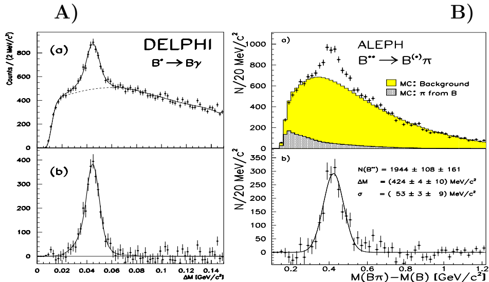
Figure 1: The distribution of the mass difference \Delta M(B^* - B) (plot A ) and \Delta M(B^{**} - B) (plot B ) before (plots a ) and after (plots b ) background subtraction. The data are represented by points with error bars. The curves on plots b ) show the results of the fit using a Gaussian distribution for the signal.
