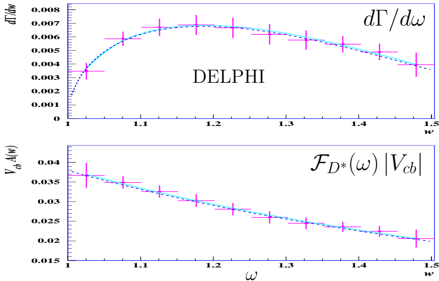
Figure 3: The differential decay width ( upper plot ) and the product of the decay form-factor \mathcal{F}_{D^*}(\omega) and the |V_{cb}| ( lower plot ) of the decay \bar{B}_d^0 \rightarrow D^{*+} l^- \bar{\nu}_l as a function of the variable \omega . The dotted (continuous) line shows the results of a fit to the data histogram neglecting (including) the statistical correlations among the bins.
