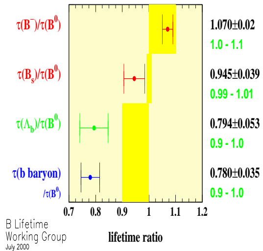
Figure 2: Average values of lifetimes of beauty hadrons together with their ratios and theoretical expectations.
