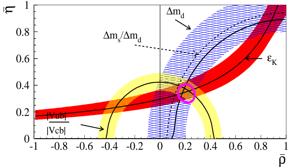
Figure 6: Selected regions in the \bar{\rho} - \bar{\eta} plane. The continuous curves represent the constraints resulting from the measurements of |V_{ub}|/|V_{cb}| , \Delta m_d , and \epsilon_K . The dotted curve corresponds to the 95% C.L. limit on the \Delta m_s/\Delta m_d . The bands surrounding the |V_{ub}|/|V_{cb}| , \epsilon_K and \Delta m_s/\Delta m_d curves represent the respective contours of 68% C.L. The allowed region (contour at 68% C.L.) is shown as a circle surrounding the region where the continuous and dotted lines cross.
