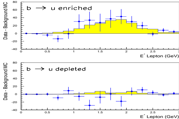
Figure 4: Background subtracted energy spectrum of leptons E_l^* , measured in the B meson rest frame, as obtained by the DELPHI for the b \rightarrow u enriched ( upper plot ) and b \rightarrow u depleted ( lower plot ) samples. The shaded histograms show the expected E_l^* distribution for the signal of b \rightarrow u semileptonic decays normalized to the fitted value of |V_{ub}|/|V_{cb}| .
