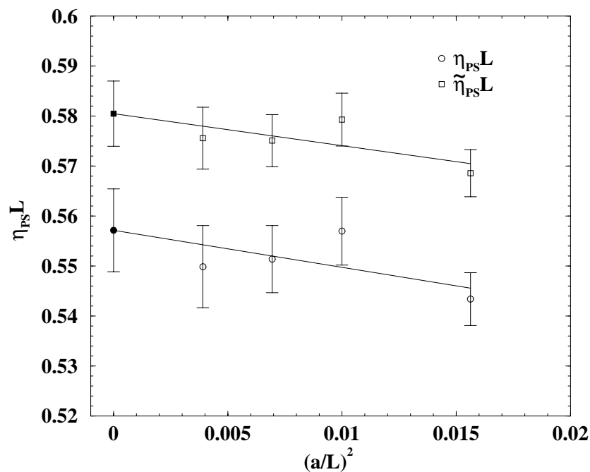
Figure 4: Scaling behaviour and continuum extrapolation for \eta_{PS}L and \tilde{\eta}_{PS}L .
