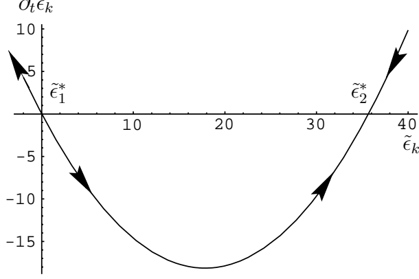
Figure 1: Fixed-point structure of the \tilde{\epsilon}_k flow equation after fermion-boson translation by hand. The graph is plotted for the threshold functions discussed in appendix E with e = 1 . Note that \tilde{\epsilon}_1^* is small but different from zero (cf. Eq. (22)). Arrows indicate the flow towards the infrared, k \rightarrow 0 .
