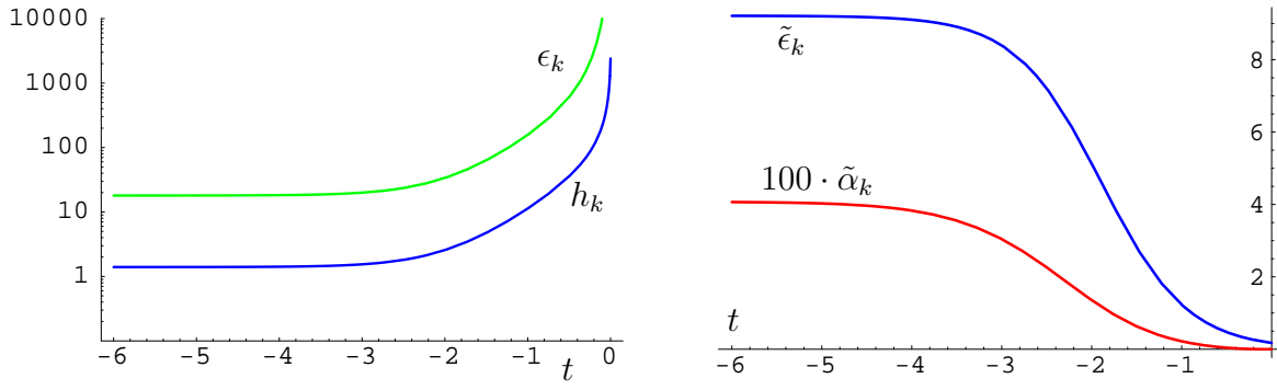
Figure 2: Flows of \epsilon_k , h_k , \tilde{\epsilon}_k and \tilde{\alpha}_k in the symmetric phase according to Eqs. (39), (40) and (46) for the initial values \epsilon_\Lambda = 10^6 , \tilde{\epsilon}_\Lambda = 0.17 \gtrsim 1/(6e^2) , e = 1 , Q_\sigma = -0.1 . For a better visualization, \tilde{\alpha}_k has been multiplied by a factor of 100. The plot of \tilde{\epsilon}_k on the right panel exhibits the crossover behavior between the fixed points \tilde{\epsilon}_1^* at small t to \tilde{\epsilon}_2^* for t \rightarrow -\infty .
