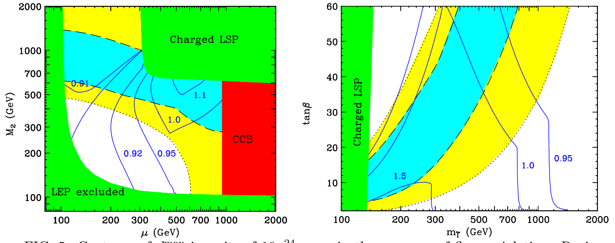
FIG. 5. Contours of d_\mu^{\max} in units of 10^{-24} e \text{ cm} in the presence of flavor violation. Regions consistent with the observed \Delta a_\mu at the 1\sigma and 2\sigma levels are also shown. On the left, m_{\tilde{t}} \approx 300 \text{ GeV} and \tan \beta = 50 , and on the right, M_2 = 300 \text{ GeV} and |\mu| = 500 \text{ GeV} . M_1 is fixed by gaugino mass unification. The excluded regions are as in Fig. 4.
