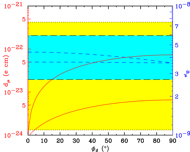
FIG. 6. Contours of d_\mu (solid) and a_\mu (dashed) as functions of \phi_\delta , the CP -violating phase present in flavor-violating slepton mass terms. In each pair of contours, the upper is for \text{Arg}(\delta_{23}^{LL}\delta_{23}^{RR}) = \phi_\delta and \delta_{23}^{LR} = \delta_{23}^{RL} = 0 , while the lower is for \delta_{23}^{LL} = \delta_{23}^{RR} = 0 and \text{Arg}(\delta_{23}^{LR}\delta_{23}^{RL}) = \phi_\delta . We fix m_{\tilde{\tau}} = 300 GeV, \tan\beta = 30 , |\mu| = 500 GeV, and M_2 = 300 GeV, and M_1 is fixed by gaugino mass unification.
