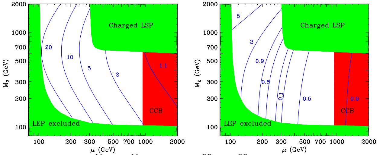
FIG. 4. The ratios \delta_{23 \tilde{B} \text{ only}}^{LL \text{ max}} / \delta_{23}^{LL \text{ max}} (left) and \delta_{23 \tilde{B} \text{ only}}^{RR \text{ max}} / \delta_{23}^{RR \text{ max}} (right). The values \delta_{23}^{\text{max}} and \delta_{23 \tilde{B} \text{ only}}^{\text{max}} are the upper bounds allowed by \tau \rightarrow \mu\gamma determined with all leading contributions and with only the Bino-mediated contribution, respectively. We fix m_{\tilde{t}} \approx 300 GeV and \tan \beta = 50 . The shaded regions are excluded by LEP, the requirement of a neutral LSP, and the condition that the vacuum not be charge-breaking.
