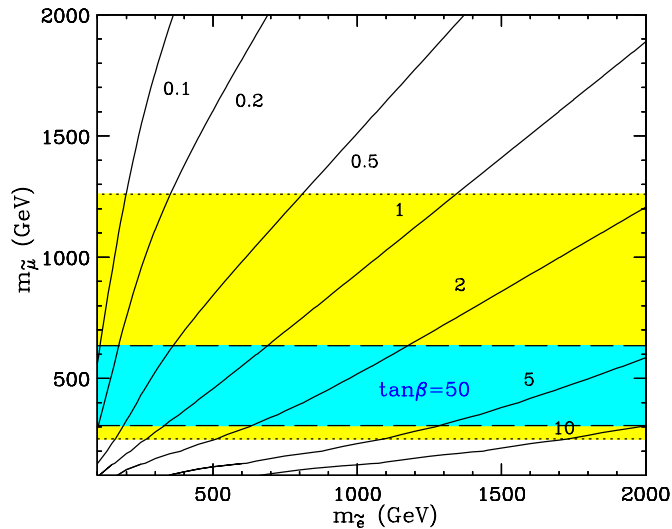
FIG. 3. Contours of d_\mu in units of 10^{-24} e cm for varying m_{\tilde{e}_R} = m_{\tilde{e}_L} = m_{\tilde{e}} and m_{\tilde{\mu}_R} = m_{\tilde{\mu}_L} = m_{\tilde{\mu}} for vanishing A terms, fixed |\mu| = 500 GeV and M_2 = 300 GeV, and M_1 = (g_1^2/g_2^2)M_2 determined from gaugino mass unification. The parameter combination \sin\phi_\mu \tan\beta is assumed to saturate the bound d_e < 4.4 \times 10^{-27} e cm. The shaded regions are preferred by a_\mu at 1\sigma and 2\sigma for \tan\beta = 50 .
