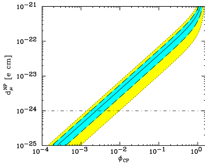
FIG. 2. Regions of the (\phi_{\text{CP}}, d_{\mu}^{\text{NP}}) plane allowed by the measured central value of |\omega_a| (solid) and its 1\sigma and 2\sigma preferred values (shaded). The horizontal line marks the proposed experimental sensitivity to d_{\mu}^{\text{NP}} .
