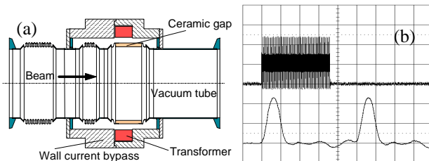
Figure 4: a) new FBCT housing. b) resulting signals with new housing.
